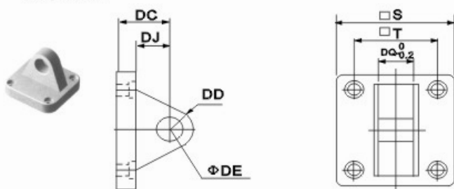
CA, Clevis
