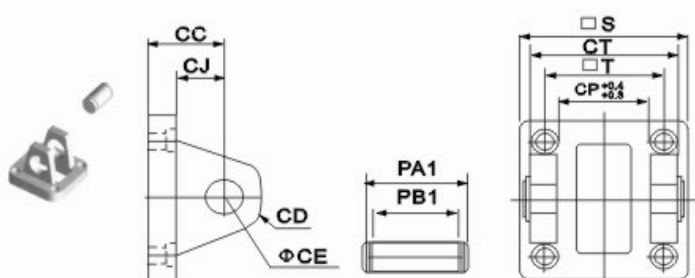
CB, Clevis
